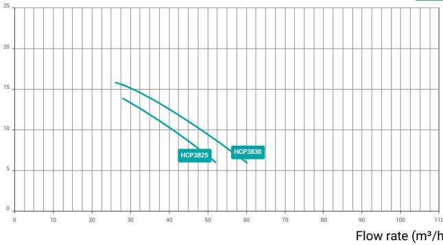
Manometric head (m)
